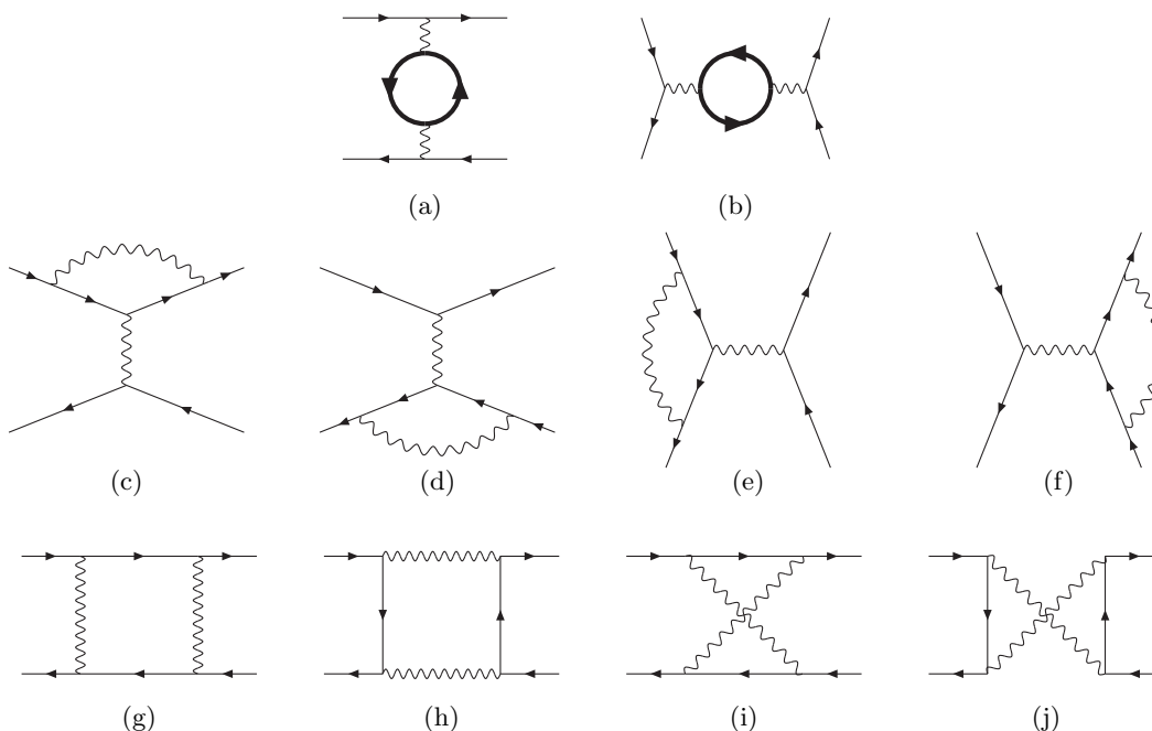
Figure 1: One-loop diagrams.
