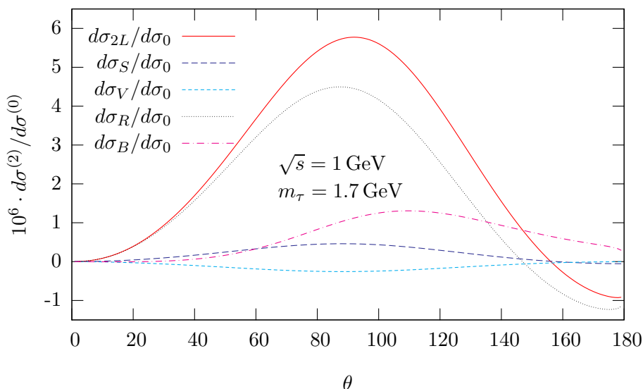
Figure 7: Self-energy (“ S ”), vertex (“ V ”), reducible plus one-loop times one-loop (“ R ”), and box (“ B ”) contributions to the two-loop \tau -lepton correction to the differential cross section of Bhabha scattering at \sqrt{s} = 1 GeV.
